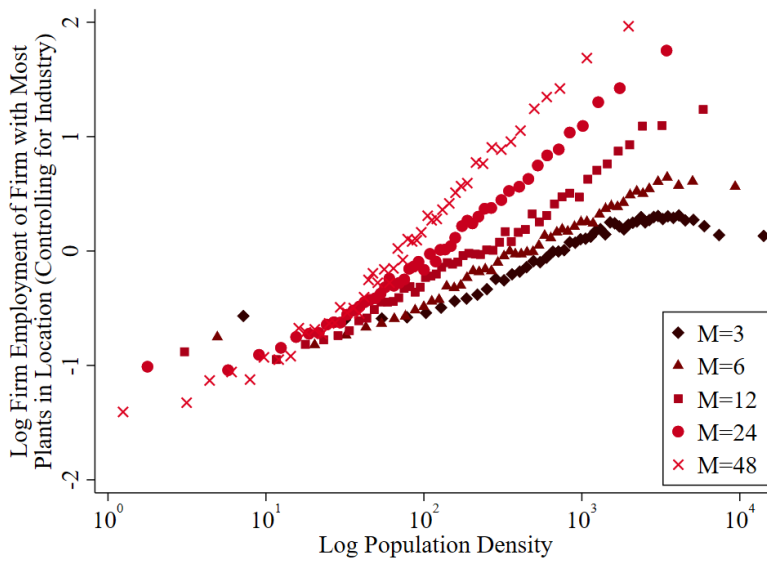
Figure C.8: The national size of the largest firm in town, non-imputed data
