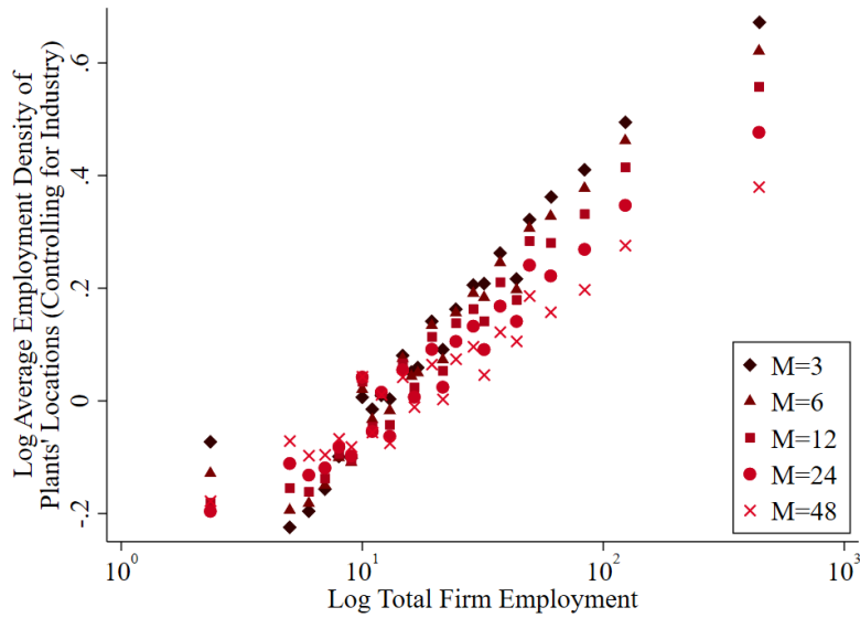
Figure C.6: Sorting in the data, non-imputed data
