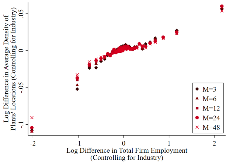
Figure C.7: Sorting over time, non-imputed data
